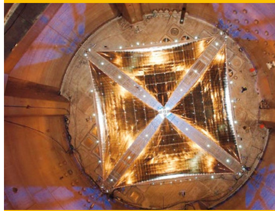
2 Deployed 20- meter solar sail on vacuum chamber floor
