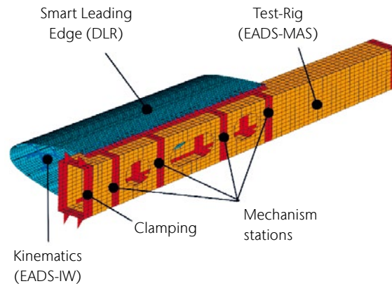
1 The finite element model of the test structure with a “smart” slat and kinematic control mechanism
