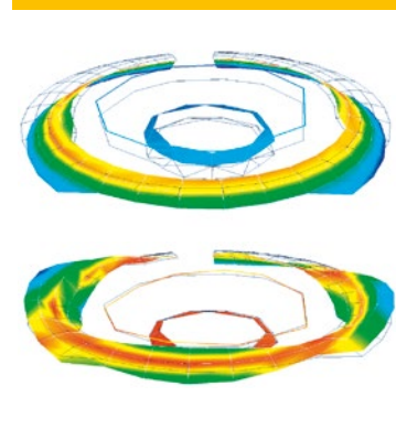
2 Operational deflection shapes at 37 Hz (a) and 353 Hz (b)
